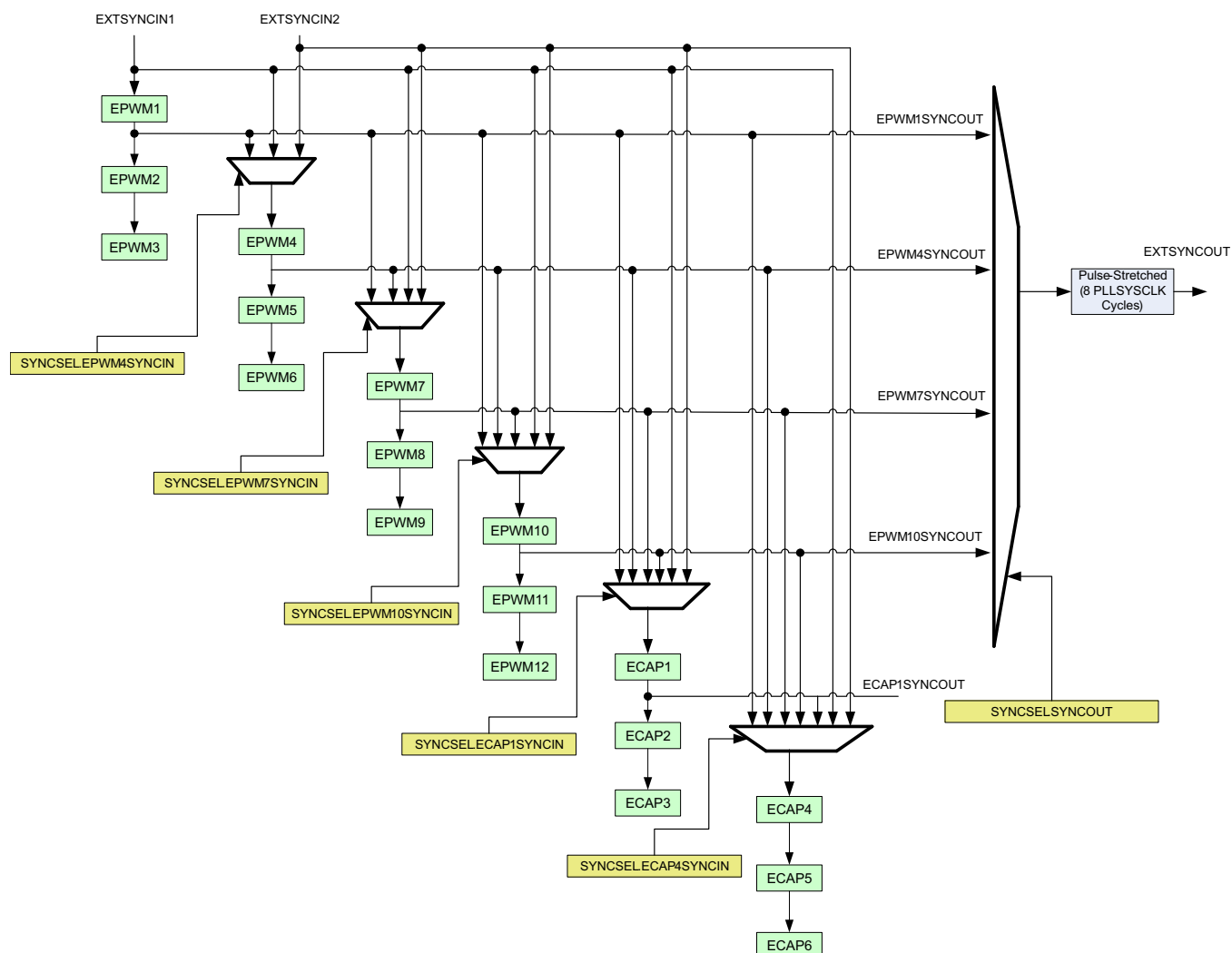
Figure 5-51. Synchronization Chain Architecture
