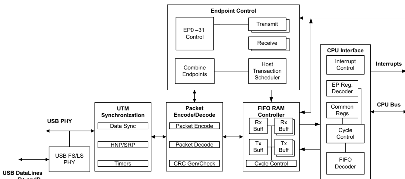
Figure 5-78. USB Block Diagram
