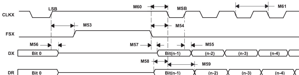
Figure 5-67. McBSP Timing as SPI Master or Slave: CLKSTP = 11b, CLKXP = 1
