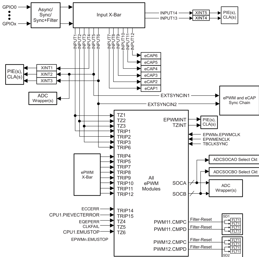
Figure 5-50. ePWM Trip Input Connectivity
