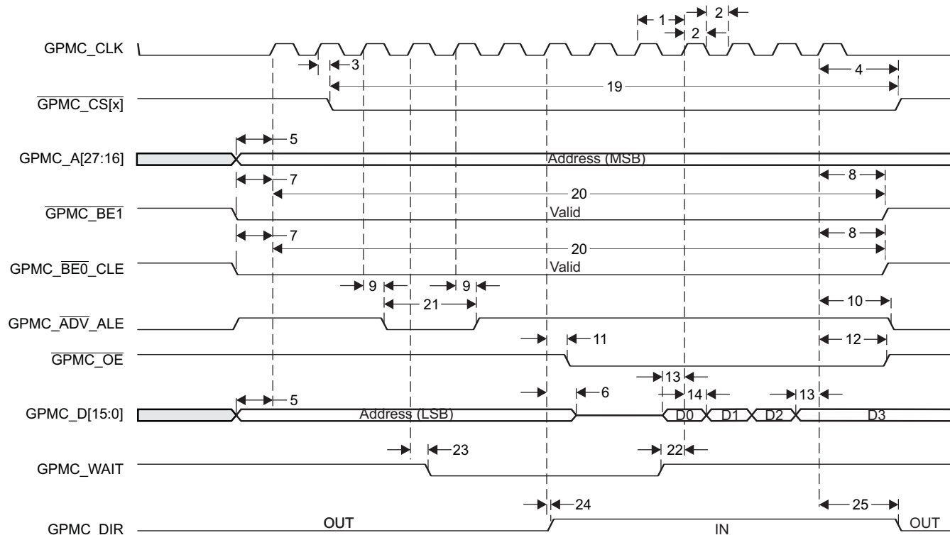
Figure 8-54. GPMC Multiplexed NOR Flash - 4x16-bit Synchronous Burst Read (GPMCFCLKDIVIDER = 0)
