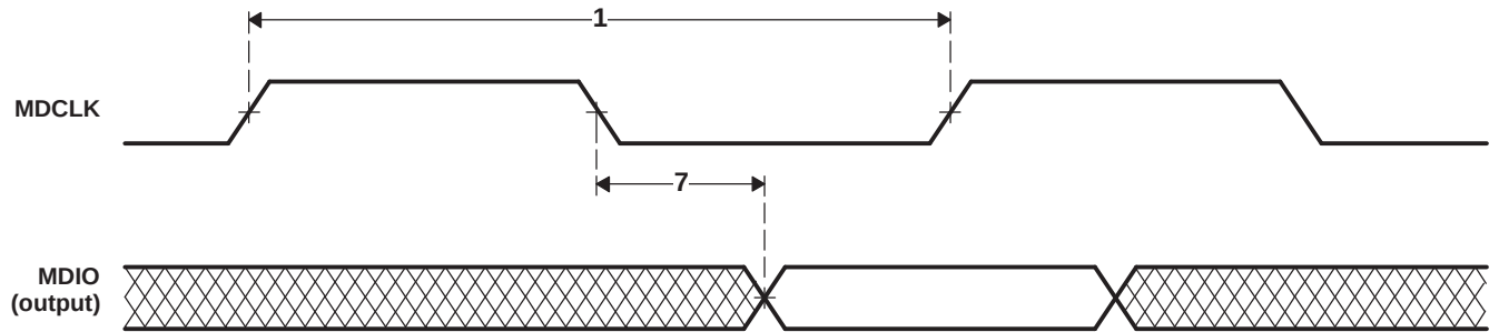
Figure 6-64. MDIO Output Timing
