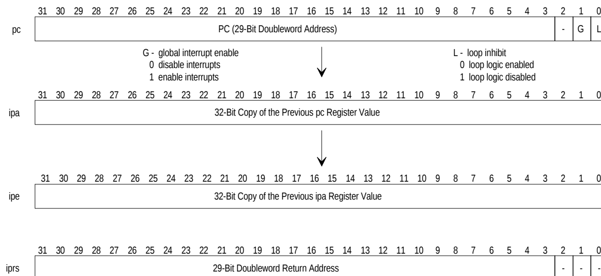
Figure 30. Pipeline Registers
