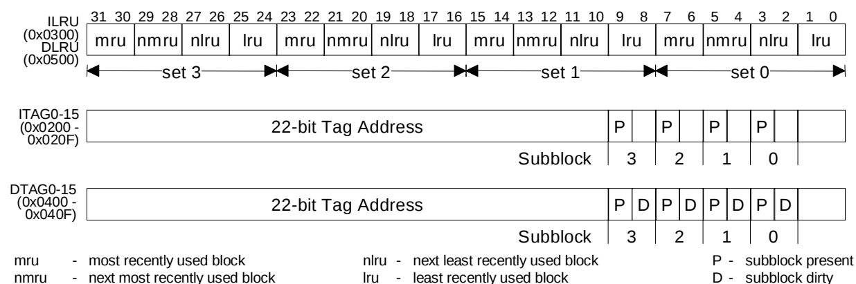
Figure 17. Cache Registers
