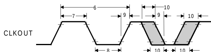
Figure 108. CLKOUT Timing
