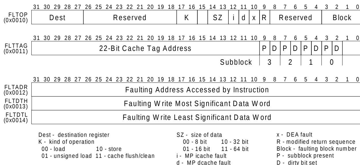
Figure 16. Memory Fault Registers
