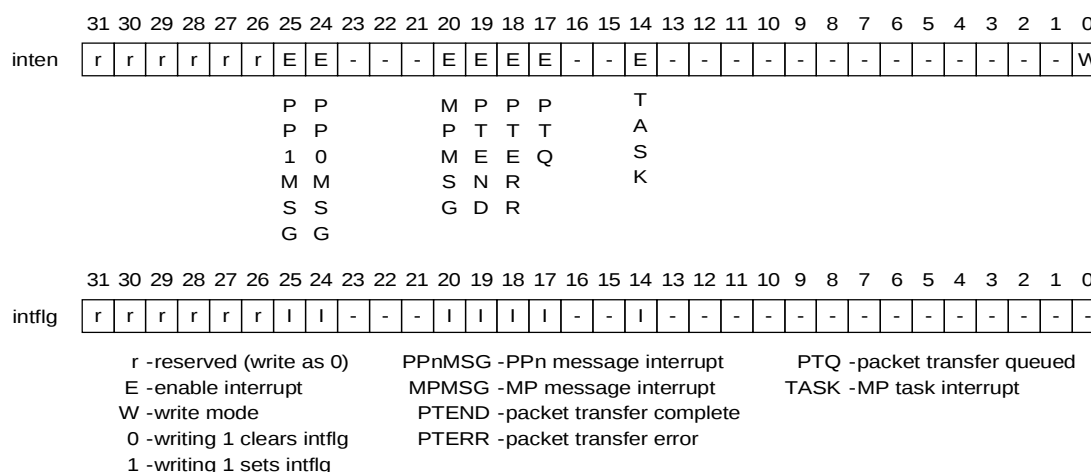
Figure 31. PP Interrupt Registers
