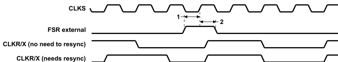
Figure 5-30. FSR Timing When GSYNC = 1
