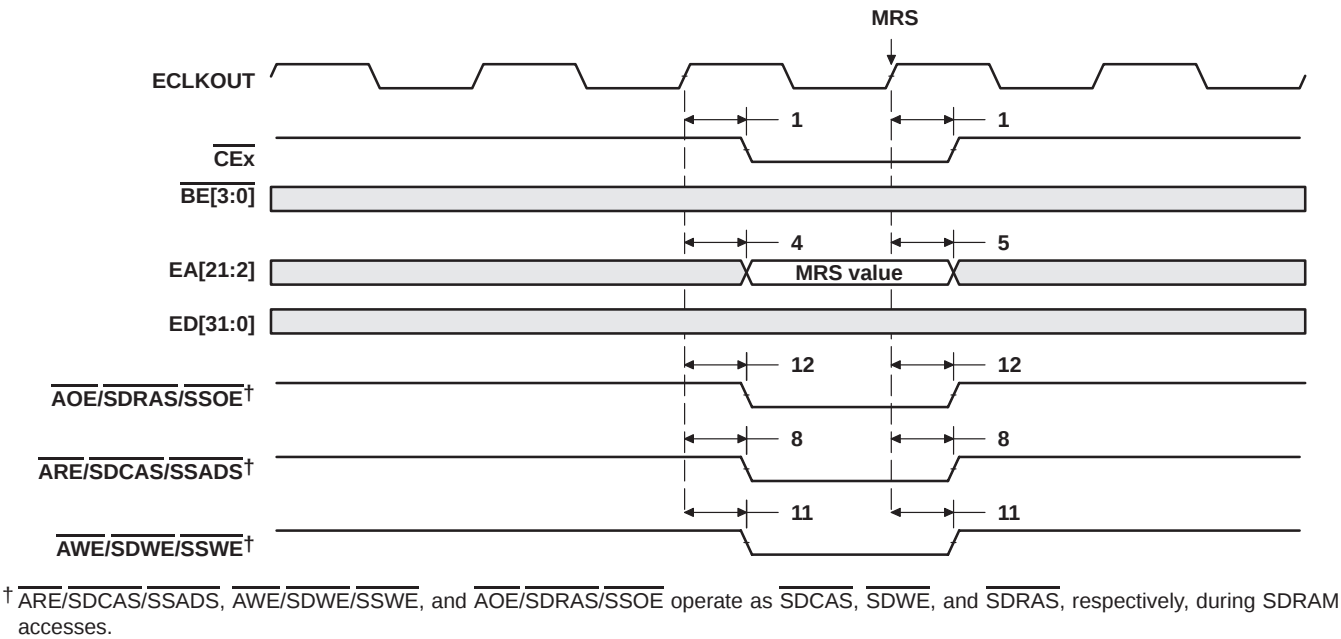
Figure 39. SDRAM MRS Command
