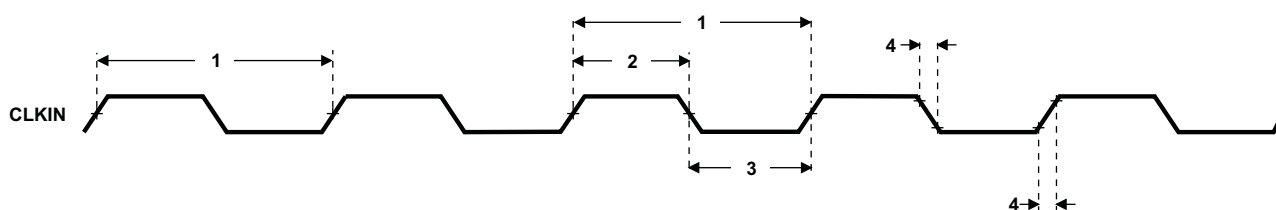
Figure 6-9. CLKIN Timing
