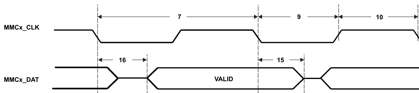
Figure 6-25. MMC/SD Data Write Timing
