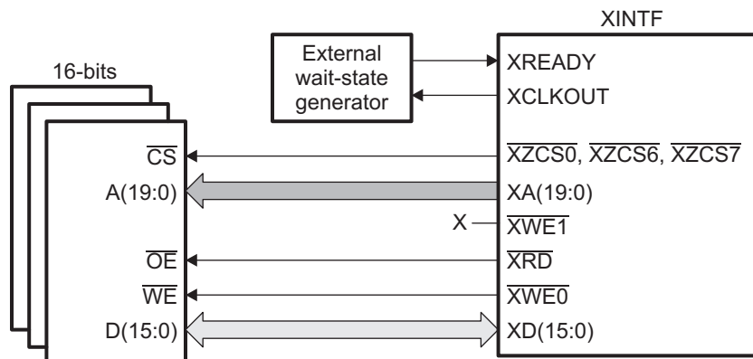
Figure 4-19. Typical 16-bit Data Bus XINTF Connections
