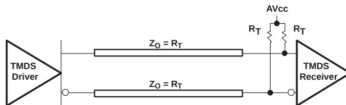
Figure 1. Termination for TMDS Output Driver
