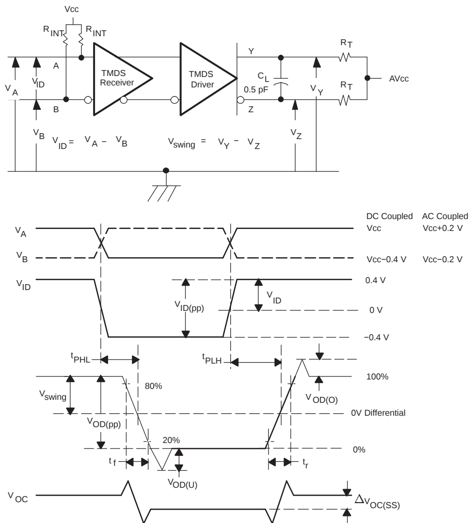
Figure 1. Termination for TMDS Output Driver
