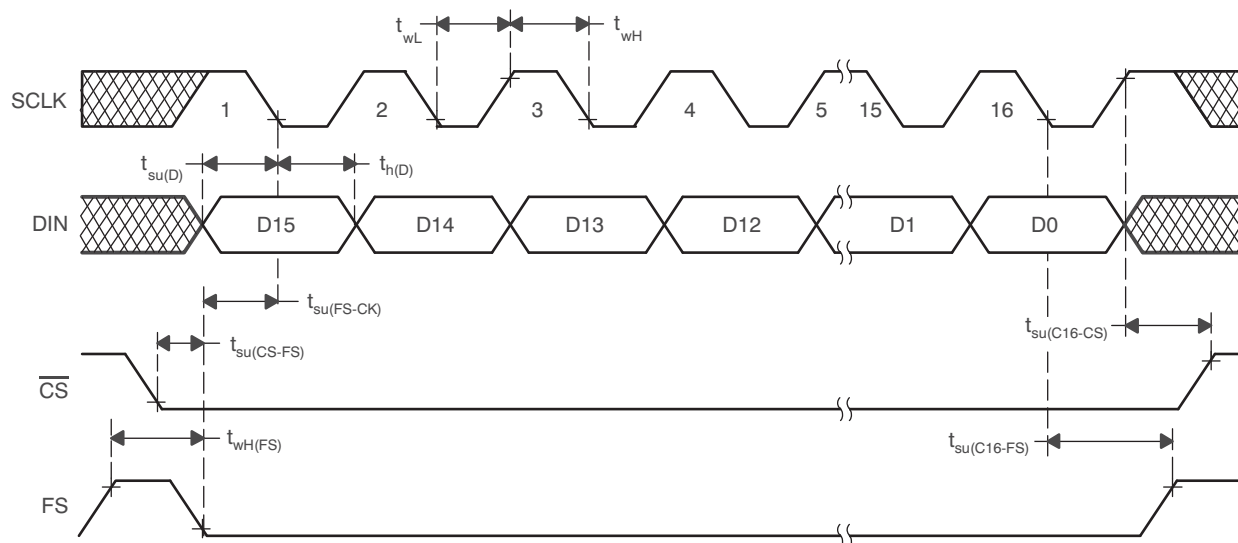
Figure 1. Timing Diagram
