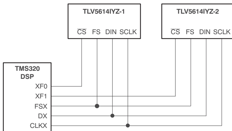
Figure 15. TMS320 Interface
