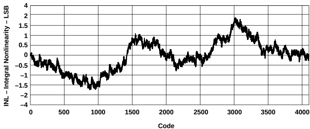
Figure 13. Integral Nonlinearity
