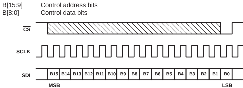
Figure 3–1. SPI Timing
