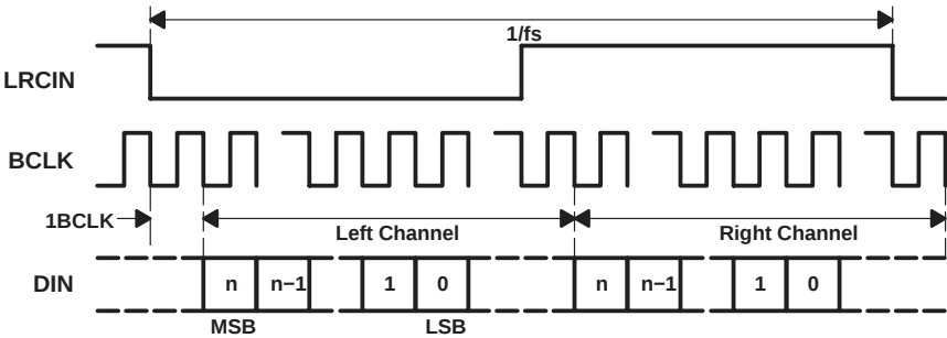
Figure 3-6. I²S Mode Timing
