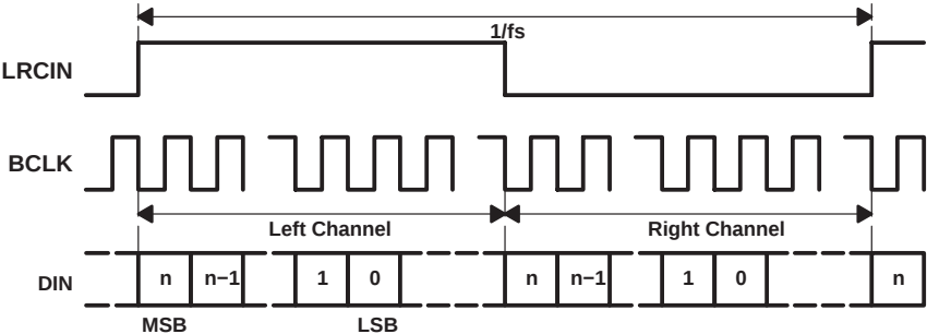
Figure 3-5. Left Justified Mode Timing
