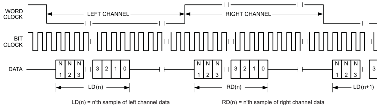
Figure 5-46. Timing Diagram for I 2 S Mode With Offset = 0 and Bit Clock Inverted
