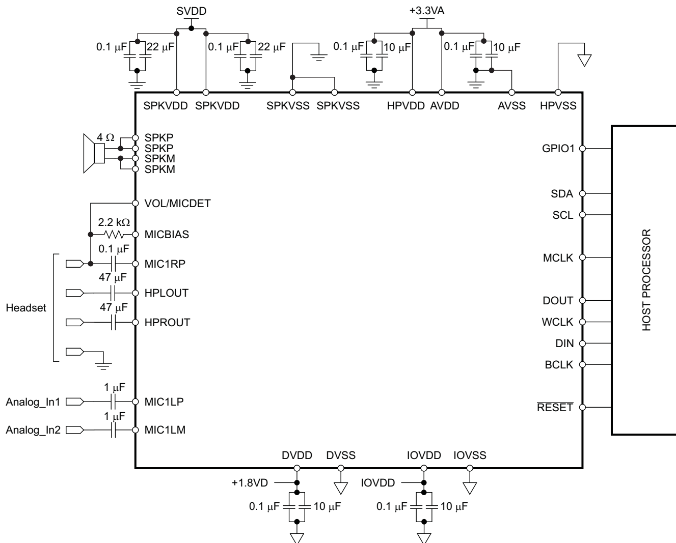
Figure 5-1. Typical Circuit Configuration
