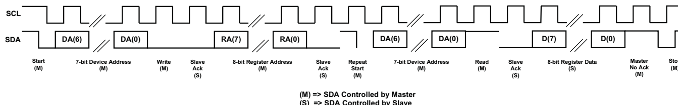
Figure 13. I 2 C Read
