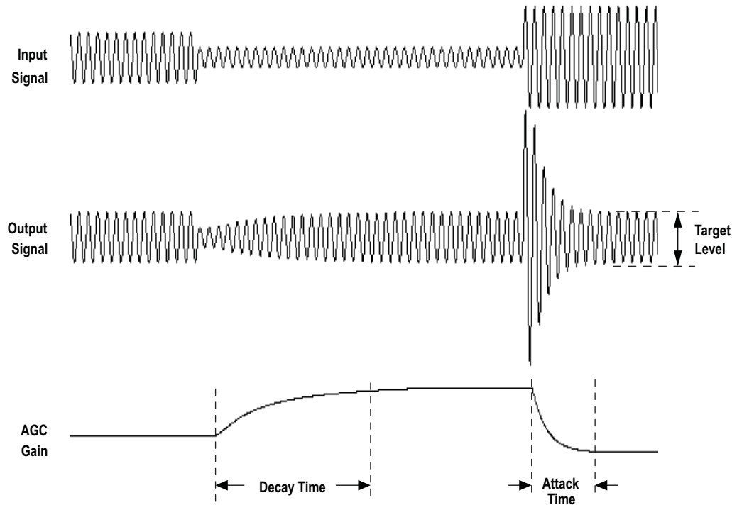
Figure 32. AGC Characteristics
