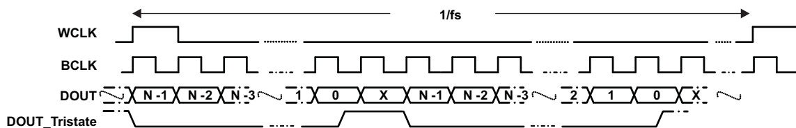
Figure 14. Both Channels Enabled, Early Hi-Z State Enabled
