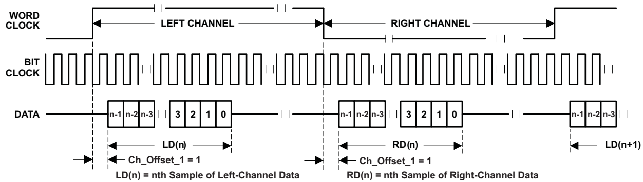
Figure 18. Left-Justified Mode With \text{Ch\_Offset}_1 = 1
