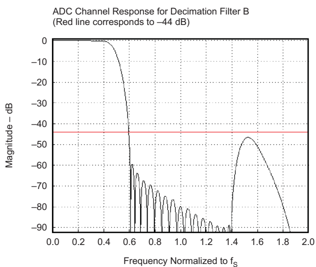
Figure 44. ADC Decimation Filter B, Frequency Response
