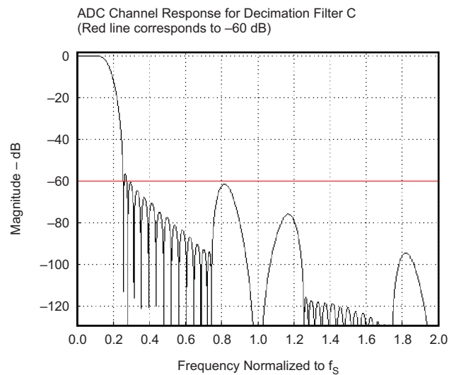
Figure 45. ADC Decimation Filter C, Frequency Response
