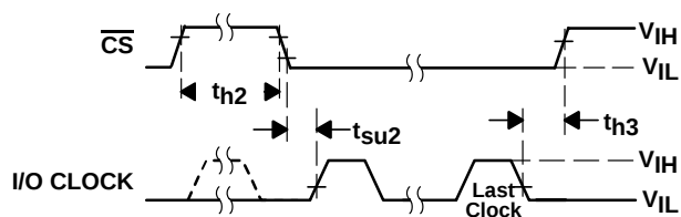
Figure 39. \overline{\text{CS}} and I/O CLOCK Voltage Waveforms
