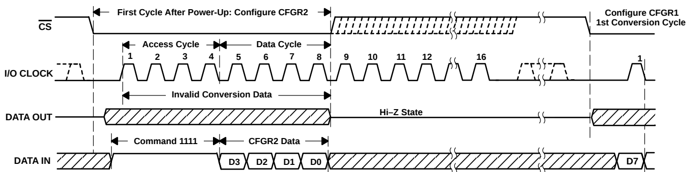
Figure 45. Timing for CFG2 Configuration
