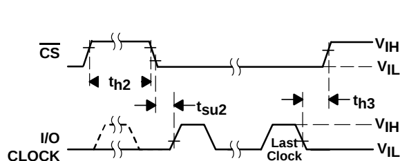
Figure 27. CS and I/O CLOCK Voltage Waveforms
