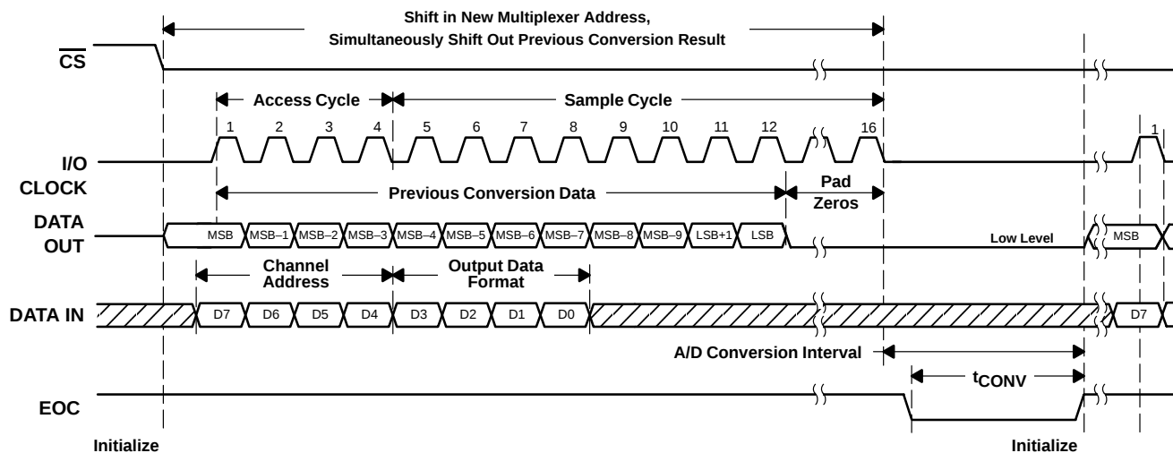
Figure 38. Timing for 16-Clock Transfer Not Using \overline{\text{CS}} With DATA OUT Set for MSB First
