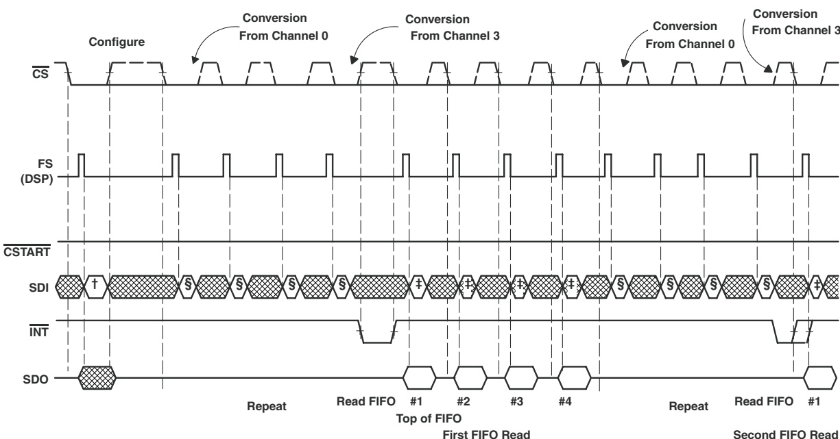
Figure 11. TLV2548 Mode 01 µp/DSP Serial Interface (Conversions Triggered by \overline{\text{CSTART}} )
