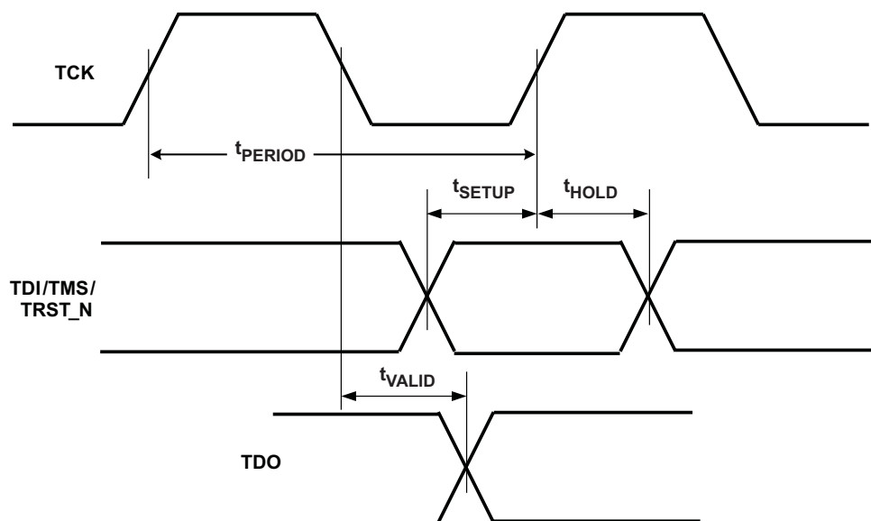
Figure 4-21. JTAG Timing
