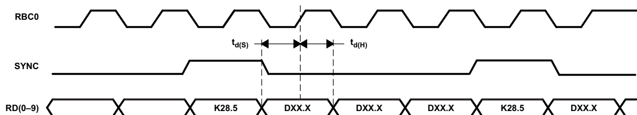
Figure 3. Synchronous Timing Characteristic Waveforms (TBI Full-Rate Mode)
