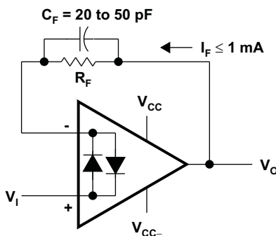
Figure 46. Voltage Follower
