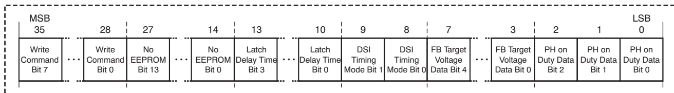
Figure 29. EEPROM1 Write Data Latch Bit Assignment
