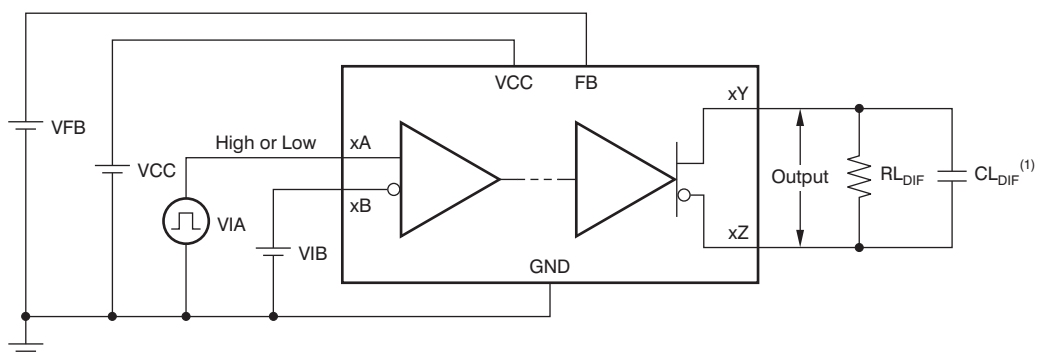
Figure 7. Rise/Fall Time and Propagation Delay Test Circuit for SDTY/Z and SCKY/Z
