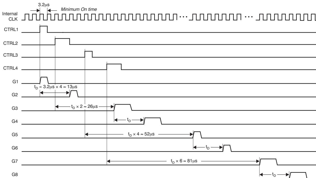
Figure 18. Built-In Phase Shift Output Sequence
