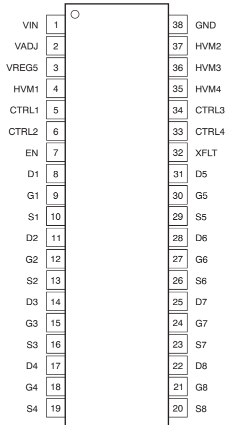
DA PACKAGE TSSOP-38 (TOP VIEW)
