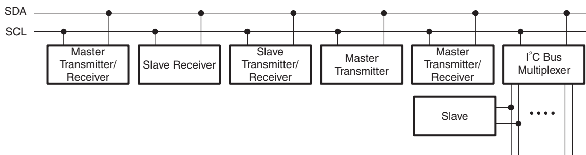
Figure 11. System Configuration
