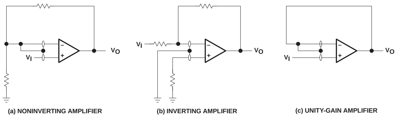
Figure 33. Guard-Ring Schemes
