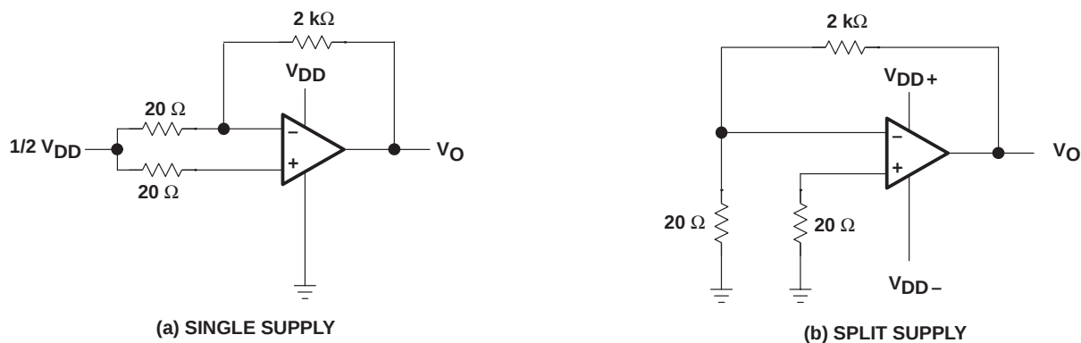
Figure 27. Noise-Test Circuit
