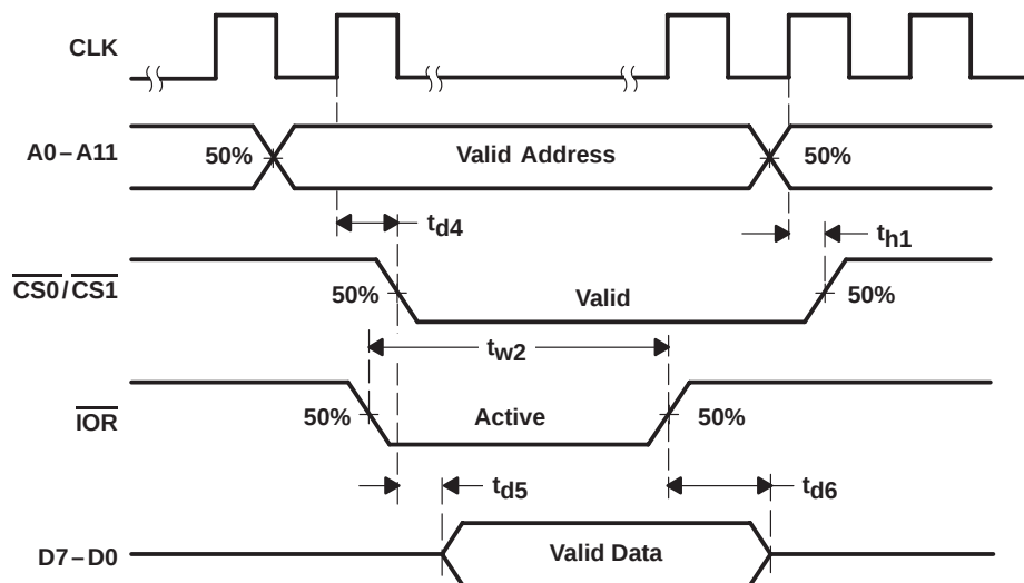
Figure 6. Read-Cycle Timing
