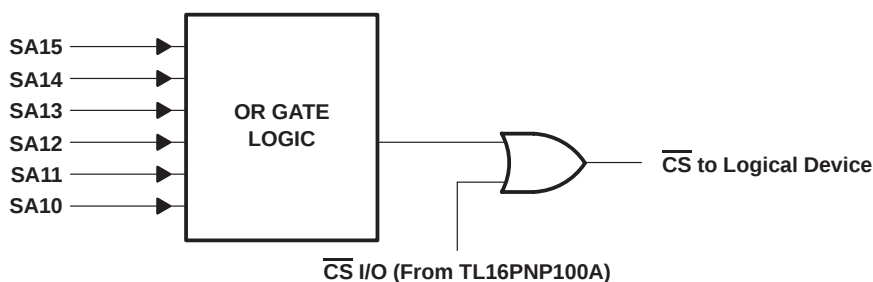
Figure 4. Gate Logic Modification
