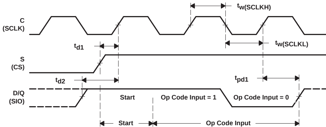
Figure 8. READ Op Code Transfer
