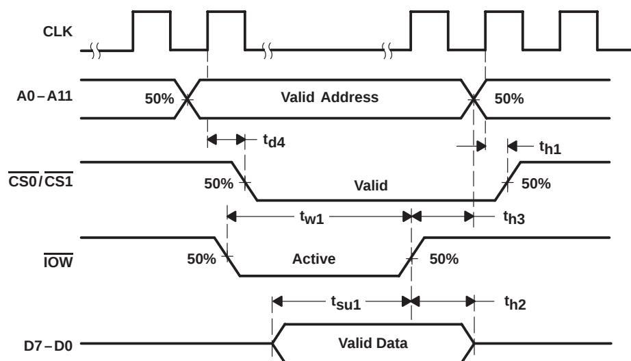
Figure 5. Write-Cycle Timing
