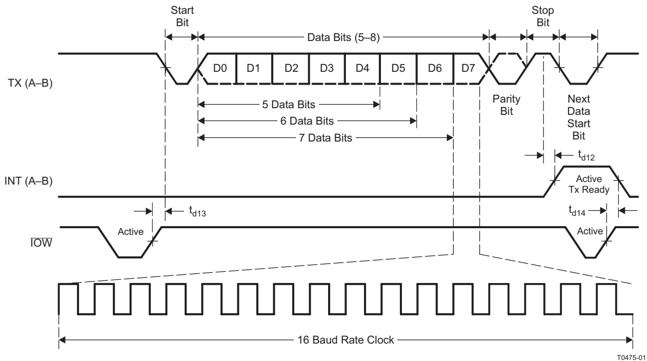
Figure 18. Transmit Timing
