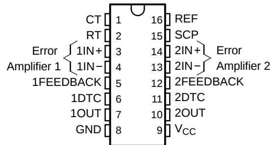
D PACKAGE (TOP VIEW)
