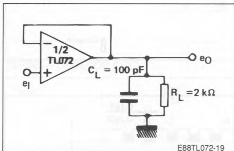
Figure 1 : Voltage follower.
