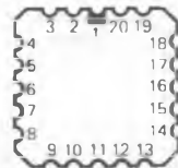
LCC20
