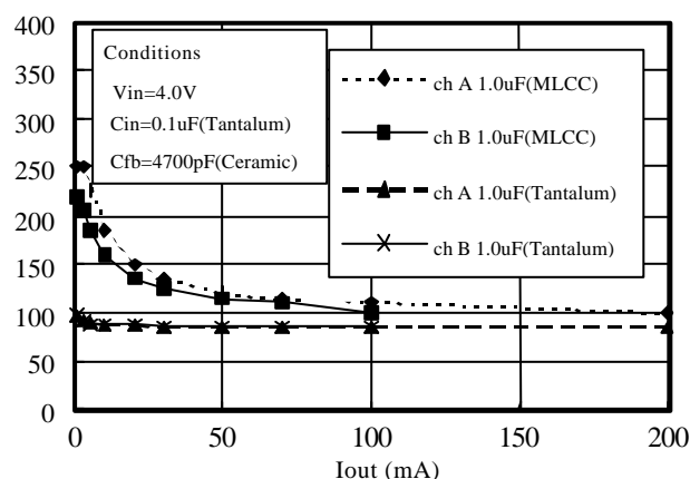
Noise (uVrms) TK74030L I_{out} VS Noise Density
