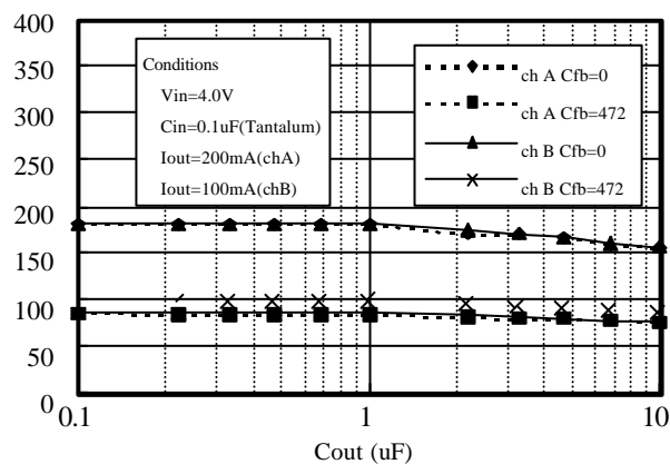
Noise (uVrms) TK74030L C_L VS Noise Density
