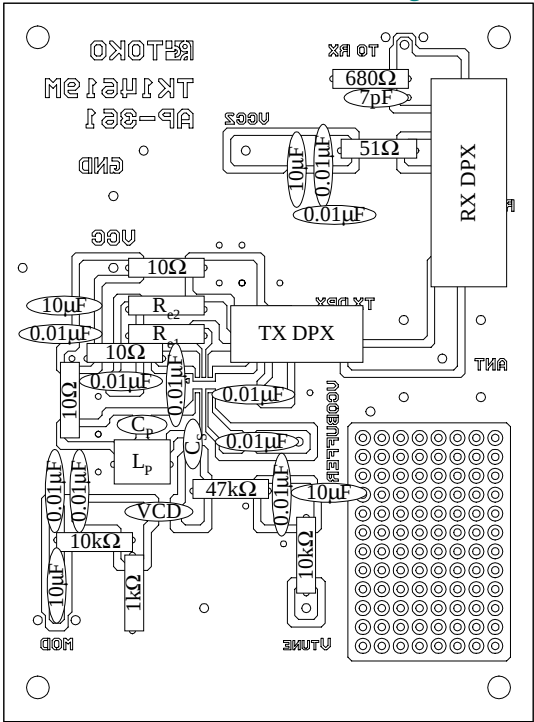
Figure 3: Component Layout View
