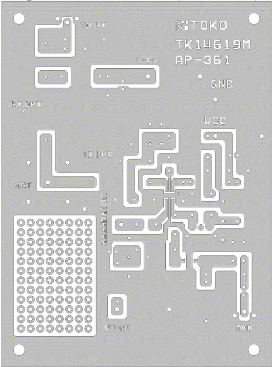
Figure 2: Solder Side View (Circuit View)
