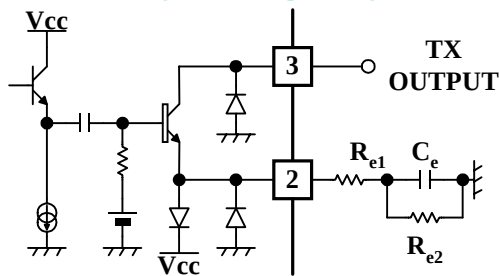
Figure 7: Output Stage
