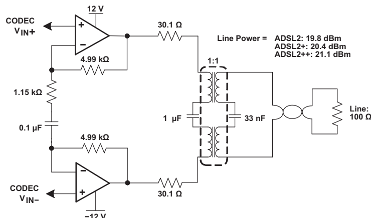
Figure 1. Typical Line Driver Circuit Using One Port of THS6184
