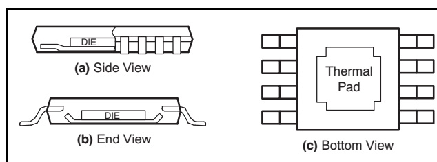
Figure 48. Views of Thermally-Enhanced Package
