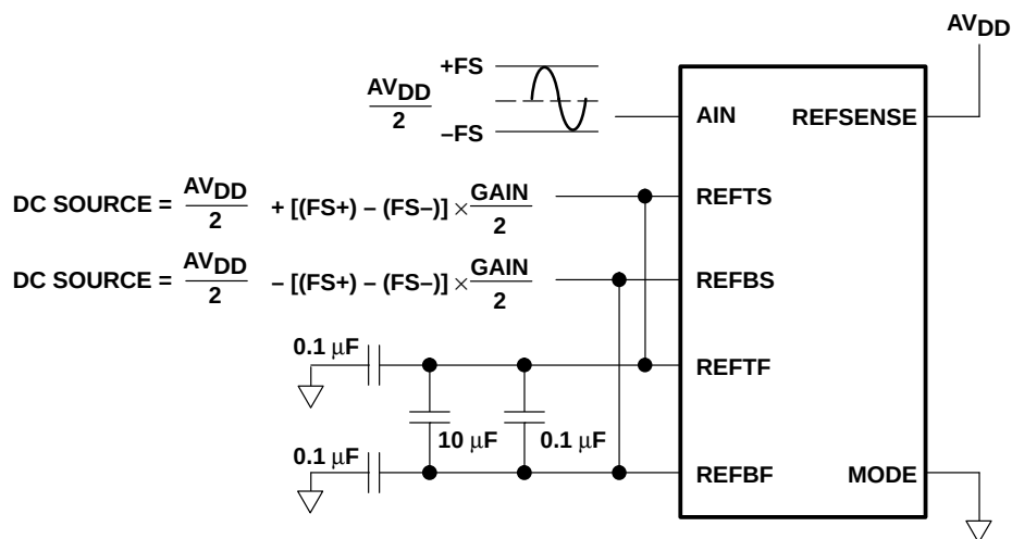
When MODE is connected to AGND, the internal reference buffer is powered down, its inputs and outputs disconnected, and REFTS and REFBS internally connected to REFTF and REFBF respectively. These nodes are connected by the user to external sources to provide the ADC reference voltages. The internal connections are designed for use in kelvin connection mode (Figure 14). When using external reference mode as shown in Figure 13, REFTS must be shorted to REFTF and REFBS must be shorted to REFBF externally. The mean of REFTF and REFBF must be equal to AV_{DD}/2 (see Figure 13).
