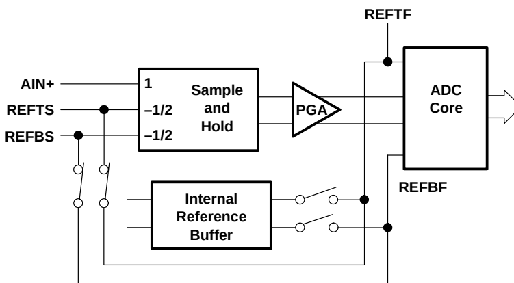
When MODE is connected to AGND, the internal reference buffer is powered down, its inputs and outputs disconnected, and REFTS and REFBS internally connected to REFTF and REFBF respectively. These nodes are connected by the user to external sources to provide the ADC reference voltages. The internal connections are designed for use in kelvin connection mode (Figure 14). When using external reference mode as shown in Figure 13, REFTS must be shorted to REFTF and REFBS must be shorted to REFBF externally. The mean of REFTF and REFBF must be equal to AV_{DD}/2 (see Figure 13).
