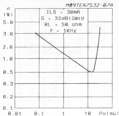
Figure 5 : Distortion Versus Output Power.
