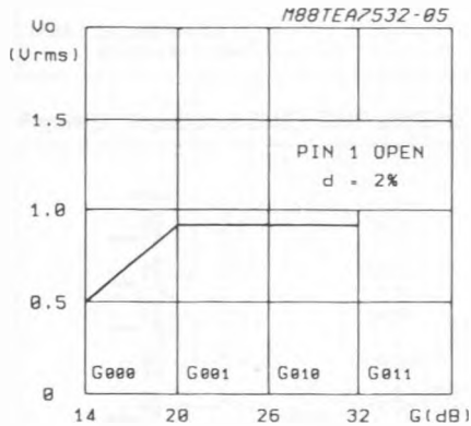
Figure 3 : AC Output Voltage Versus Amplifier Gain.
