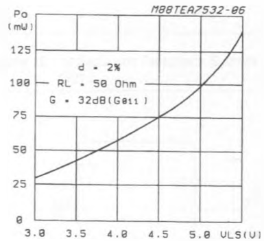
Figure 4 : Power Available on Loudspeaker Versus V LS Typical Curve.
