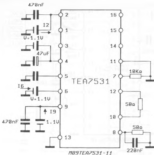
Figure 8 : Impedance ZMIC, ZINP and Zin2.
