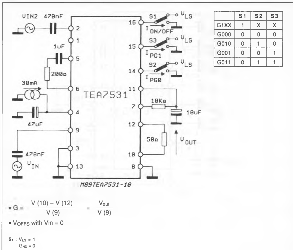
Figure 7 : Loudspeaker Amplifier : Gain/Distortion/Output Offset.
