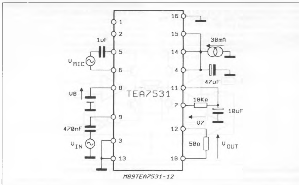
Figure 9 : Antiacoustic Feedback System at G011.
