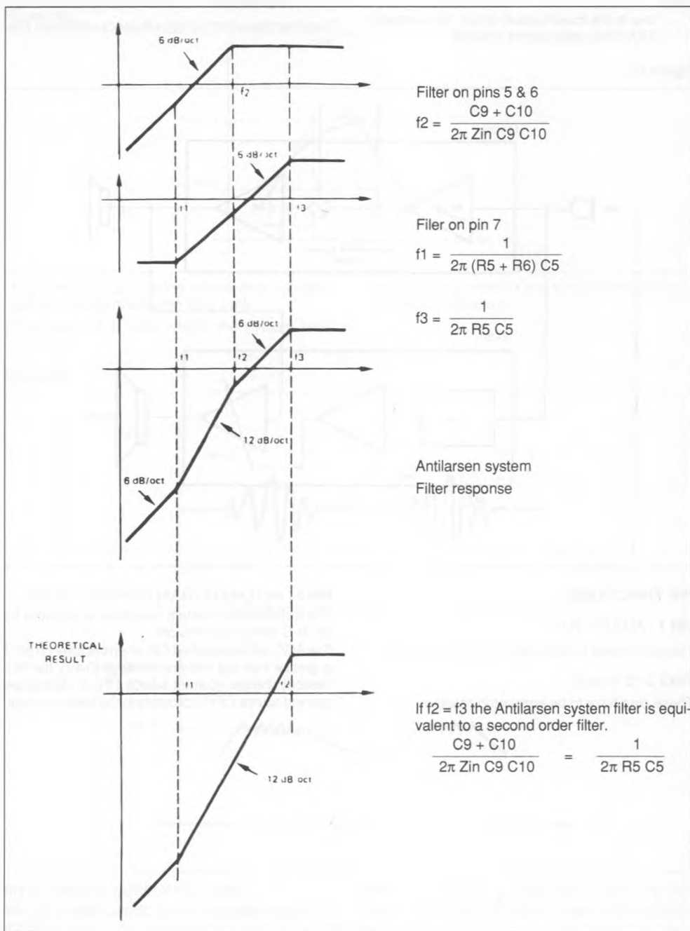
Figure 16 : Antilarsen System Filter Response.
