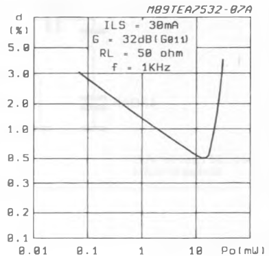
Figure 4 : Distortion versus Output Power.
