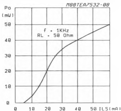
Figure 5 : Output Power versus Supply Current.
