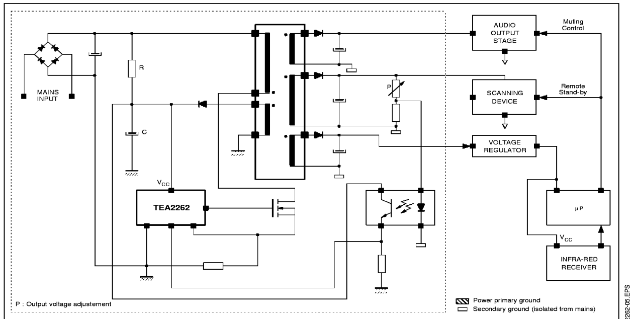
Figure 2 : Secondary Regulation (with optocoupler)
