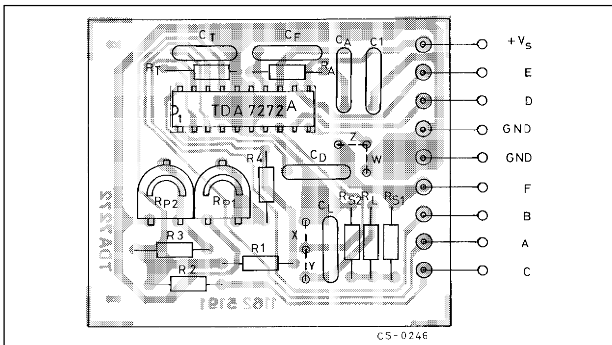
Figure 23: P.C. board and components layout of the circuits of Figg. 20, 21, 22.
