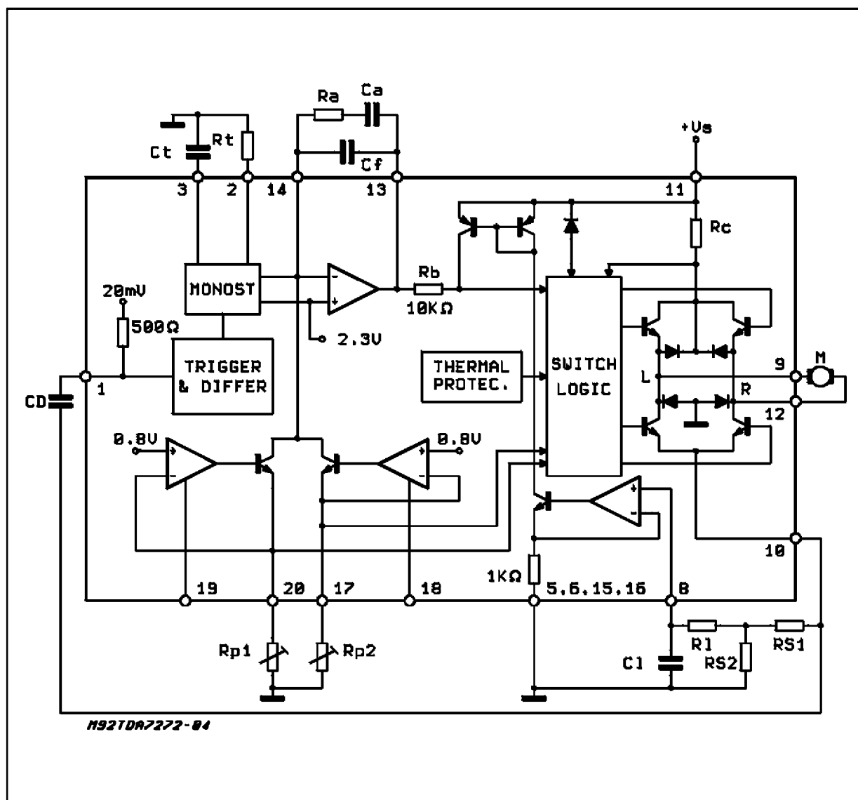
Figure 2: Application Circuit.
