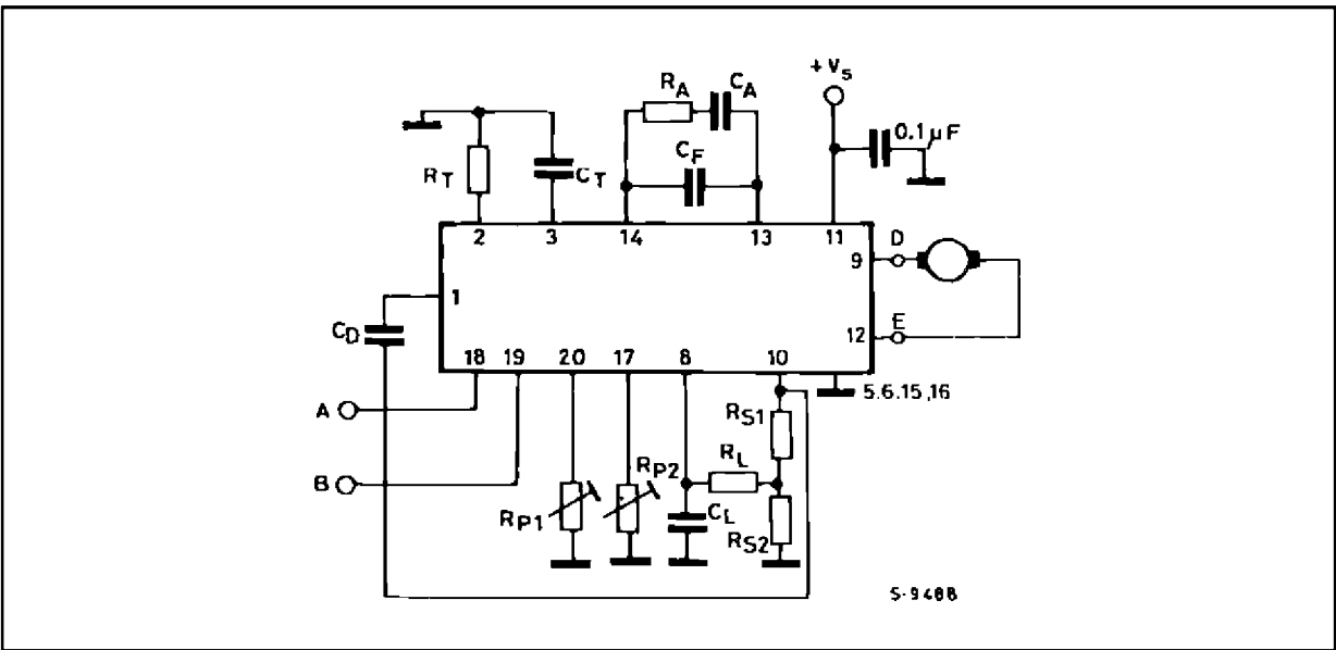
Figure 20: Typical application.
