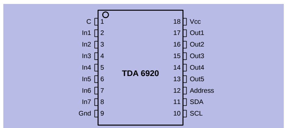
Figure 3-2 Pin Configuration P-DIP-18
