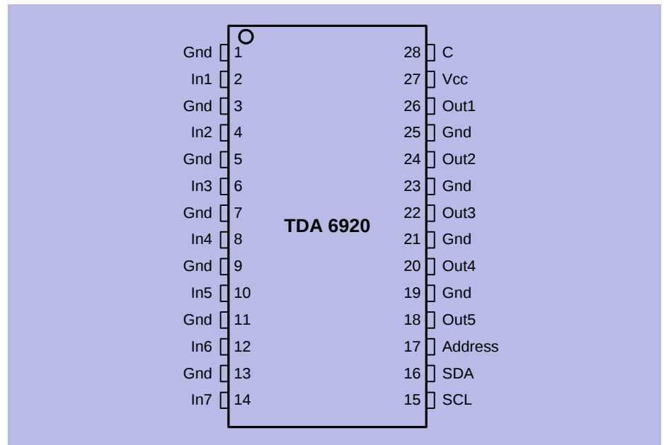
Figure 3-1 Pin Configuration P-DSO-28
