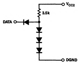
Figure 3. Equivalent Digital Input Circuit
