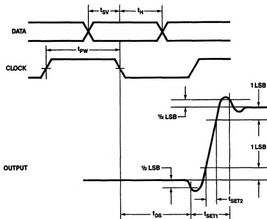
Figure 1. Timing Diagram
