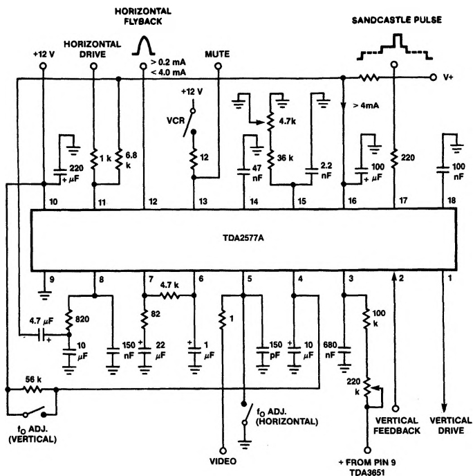
Figure 4. Typical Application Circuit Diagram; for Combination of the TDA2577A with the TDA3651 (see Figure 6)
