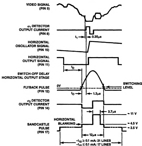
Figure 3. Timing Diagram of the TDA2577A
