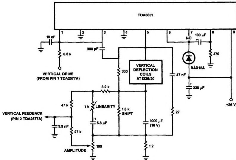
Figure 6. Typical Application Circuit Diagram of the TDA3651 (Vertical Output) When Used in Combination With the TDA2577A (90°C Application)
