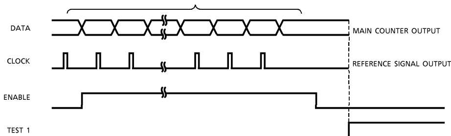
DIAGRAM 2. Test mode (Mode 1, 2)
