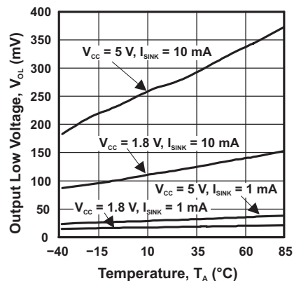
I/O LOW VOLTAGE vs TEMPERATURE
