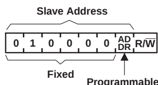
Figure 4. TCA6408A Address
