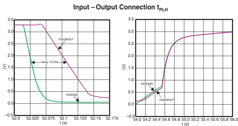
Figure 15. System With Disparate V CC Voltages
