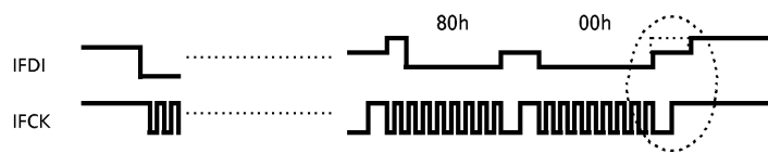
Fig.4 Timing at the Time of Command Transmission
