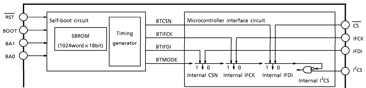
Fig.1 Self-Boot System
