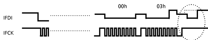
Fig.5 Timing at the Time of Self Boot Command Transmission
