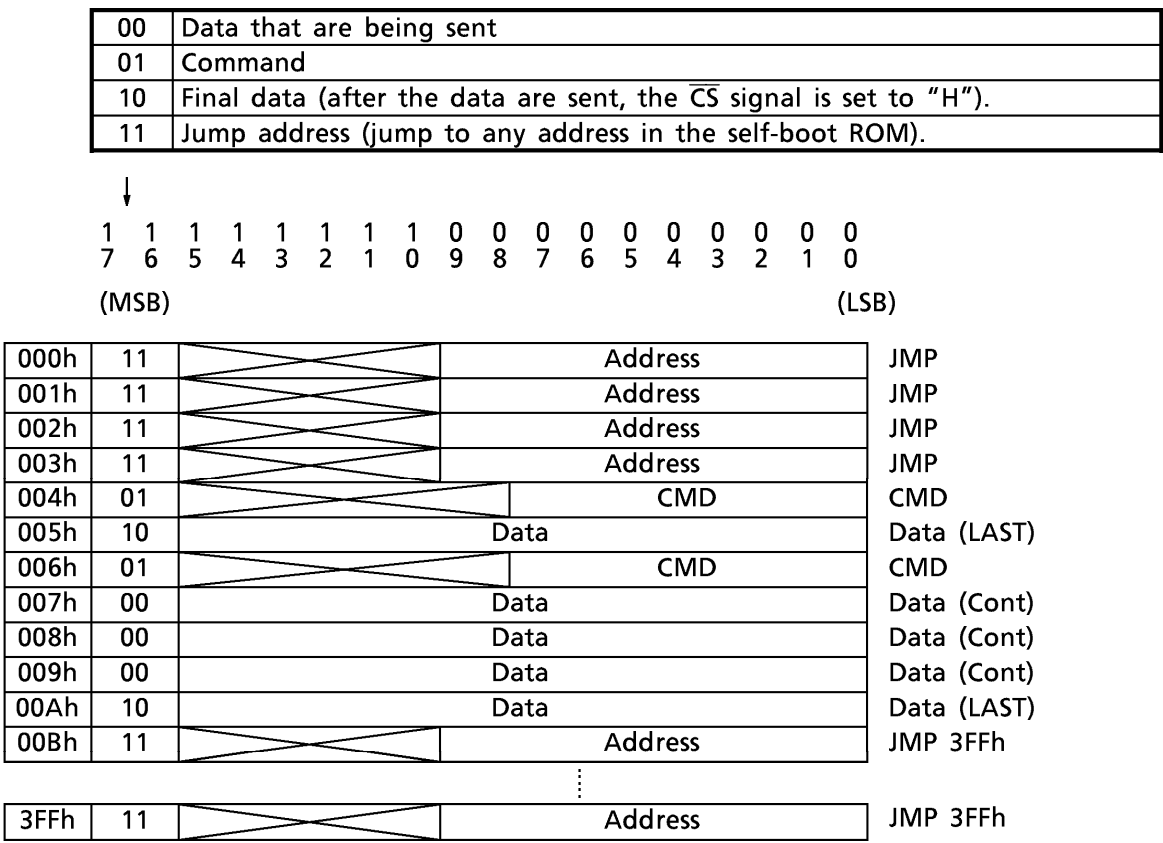
Fig.2 Boot ROM Format and Example
