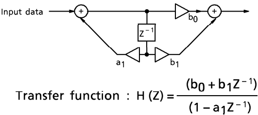
Fig.4 IIR Digital De-emphasis Filter
