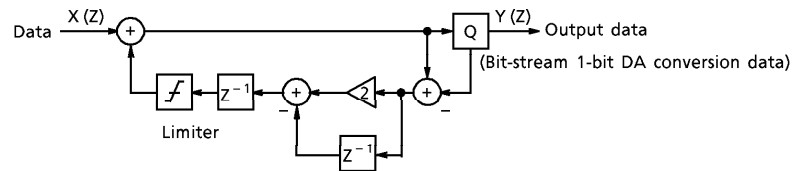
Fig.9. \Sigma - \Delta modulation DA converter
