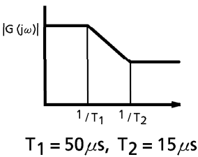
Fig.5 Filter Characteristics
