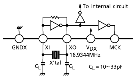
Use a crystal with a low CI value and favorable start-up characteristics. Fig.1 Crystal Oscillator Circuit Configuration (when in the 384fs mode)
