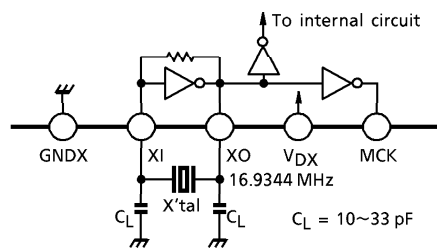
Use a crystal with a low CI value and favorable start-up characteristics. Fig. 1 Crystal Oscillation Circuit Configuration (when in the 384 fs mode)
