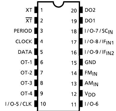
Top View DIP-20PIN / SOP-20PIN
