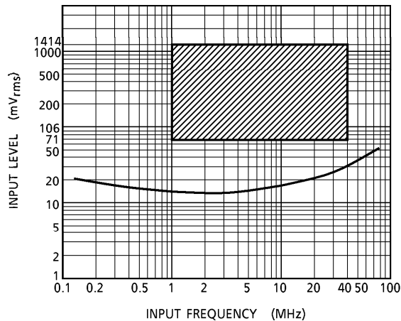
AM IN (HF) Frequency Characteristics
