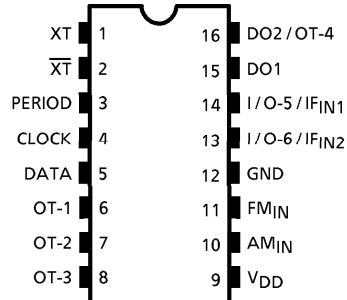
Top View DIP-16PIN / SOP-16PIN
