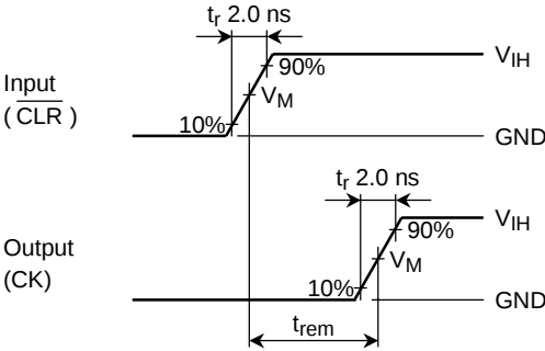
Figure 6 t_{rem}
