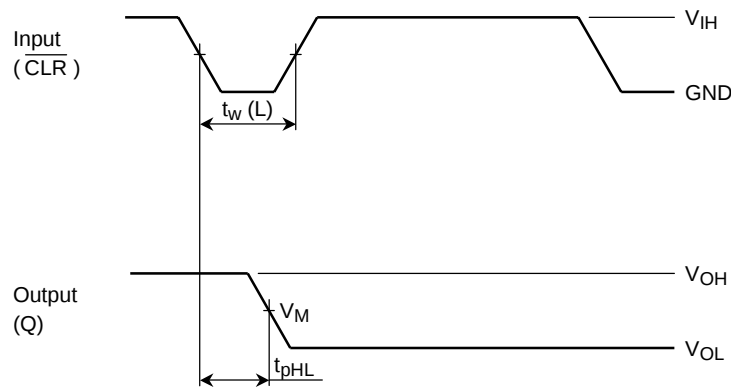
Figure 3 t_{pLH} , t_{pHL}
