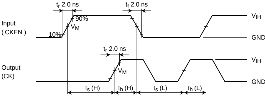
Figure 5 t_s , t_h
